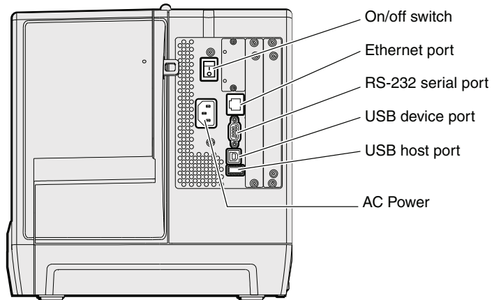
Back View of the PM43 Printer
