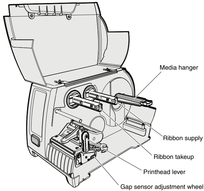
Internal View of the PM43 Printer
