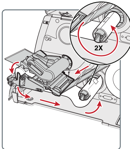
Route the Liner Around a Cardboard Core
